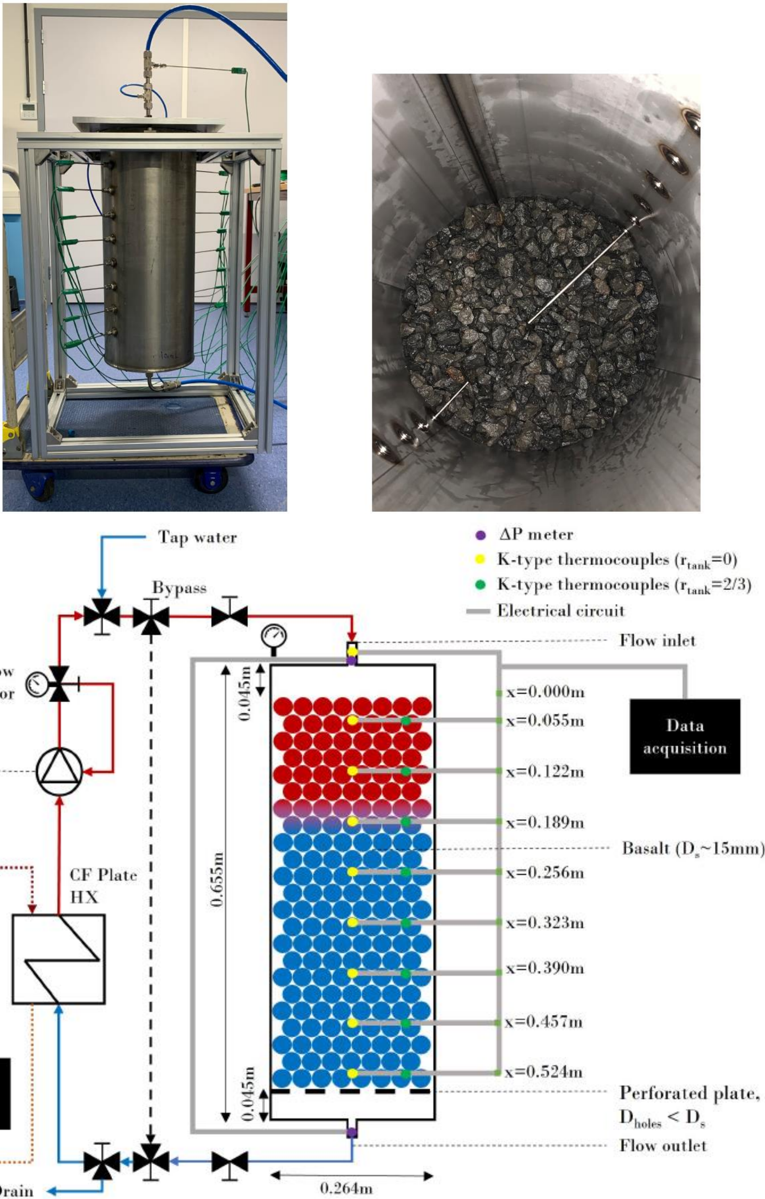
Figure 1: Experimental setup from thesis of MSc. Mark Willemsz (2023)
