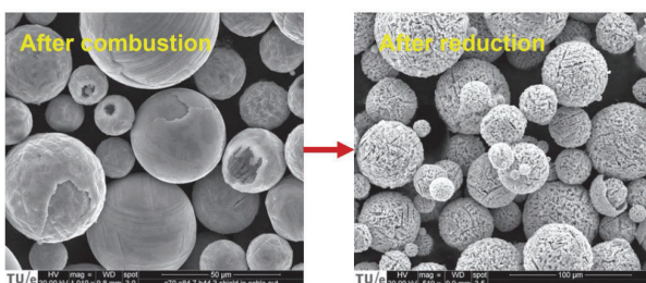
Figure 1: SEM images of combusted iron (left) and direct reduced iron (right) [1]
