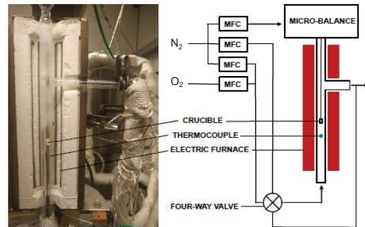
Figure 2. Diagram of the thermogravimetric experimental setup [2]
