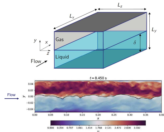
Figure 3: DNS of turbulent stratified flow. (a) schematic of the computational domain. (b) A snapshot of the interface and streamwise flow field at z=0 .
