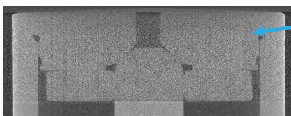
Figure 2: CT-scan showing the insides of the H2 injector. Note the bullet shaped needle closing of the exit hole in the middle.
