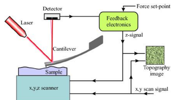
Figure 1: Principles of atomic force microscopy [1]
