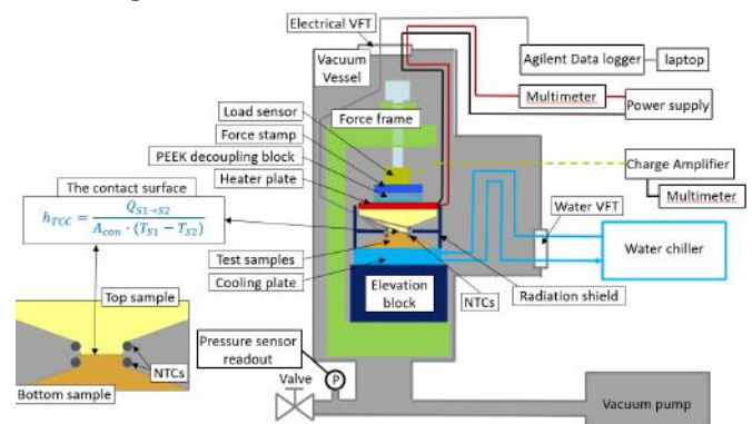
Fig 1b: Schematic representation of test setup
