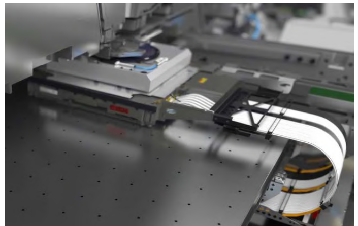
Fig 1a: Hoses in high precision motion stage (courtesy: ASML)
