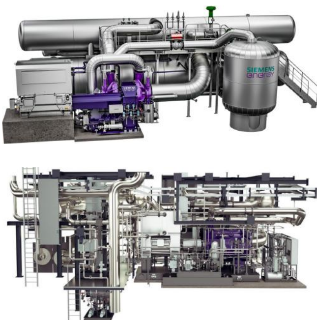
Fig. 1. Typical industrial heat pumps and their integration for cooling purposes (from Siemens Energy).
